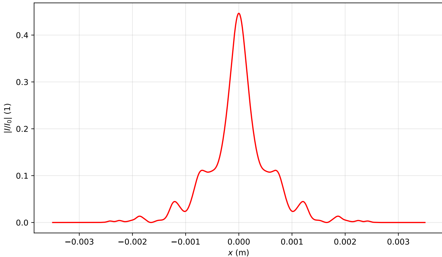
Intensity profile I(x, y = 0, z = 2.149)/I_0 , P_{in}=5.5P_{cr} , artificial time
